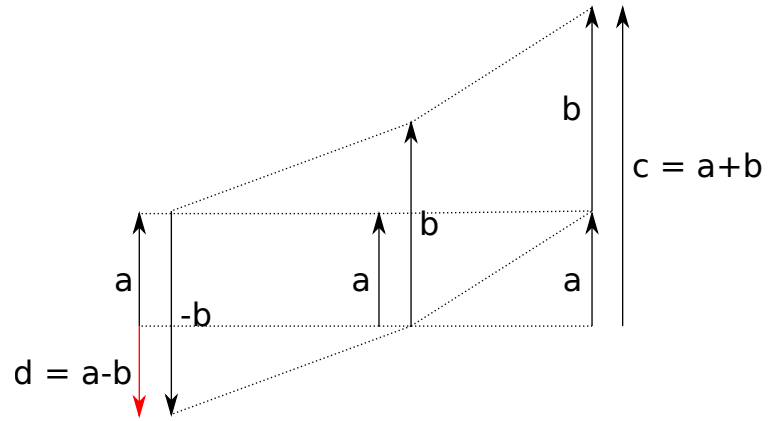
FIG. 1: Vector addition and subtraction
